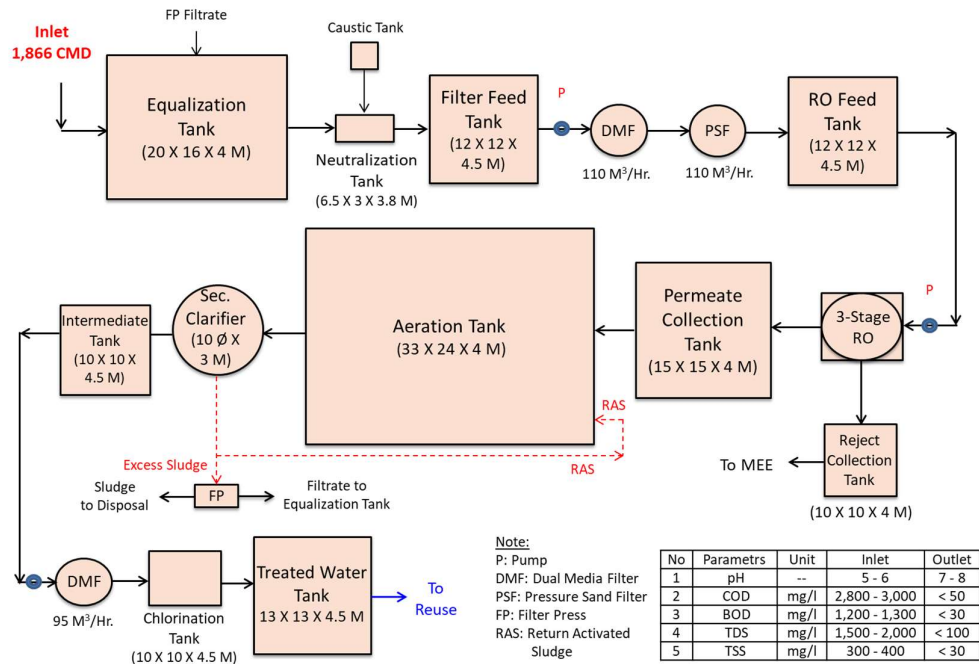
Figure 4. Flow Chart of Upgradation in Existing Distillery CPU
