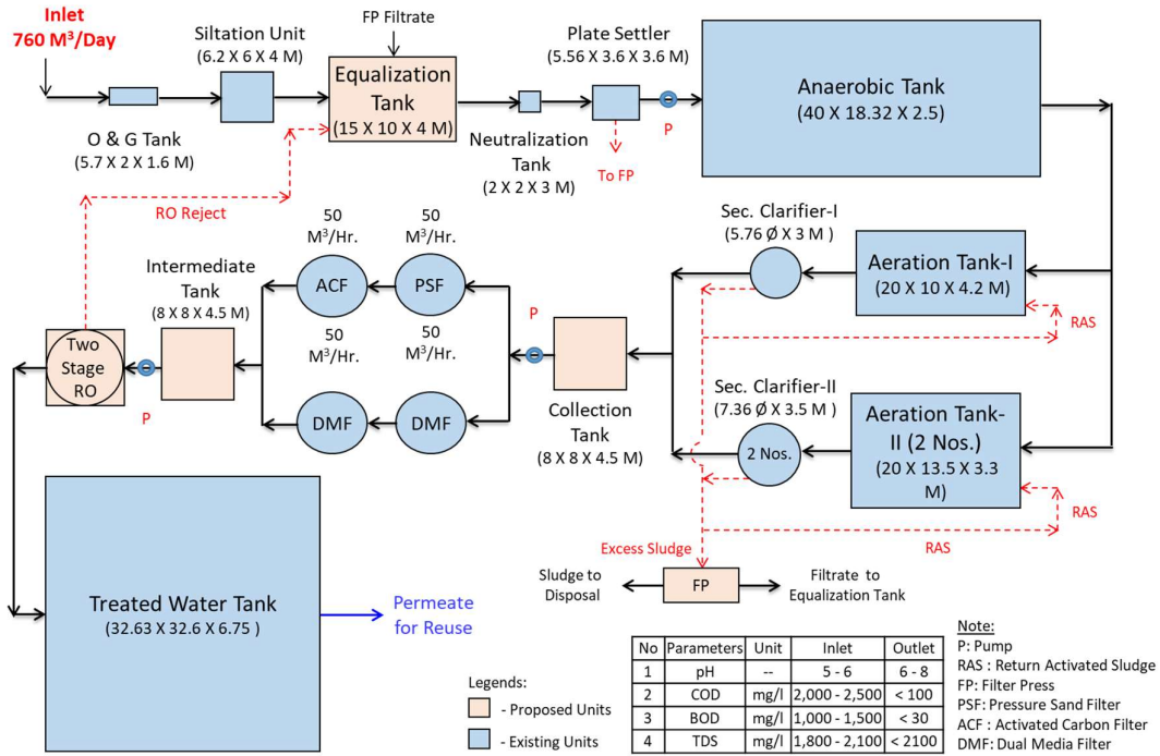
Figure 3. Flow Chart of Upgradation in Existing Sugar Factory ETP
