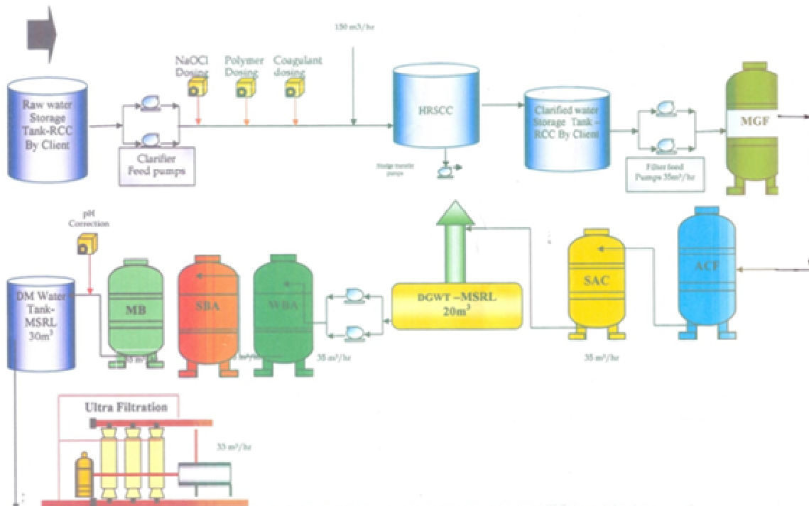
Figure 2.4 Flow Diagram of DM plant & detailed process
