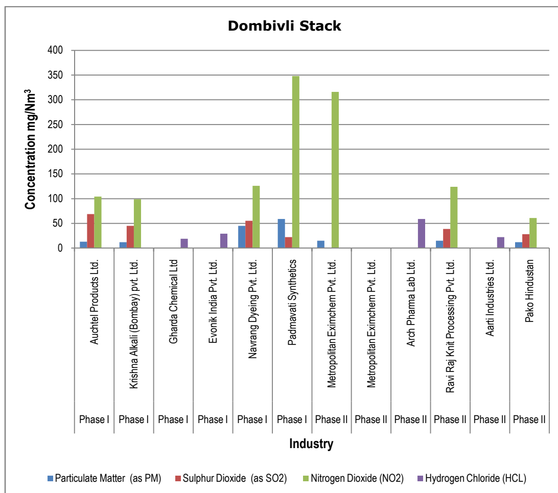
Graphs: Stack Monitoring for Dombivli MIDC:
