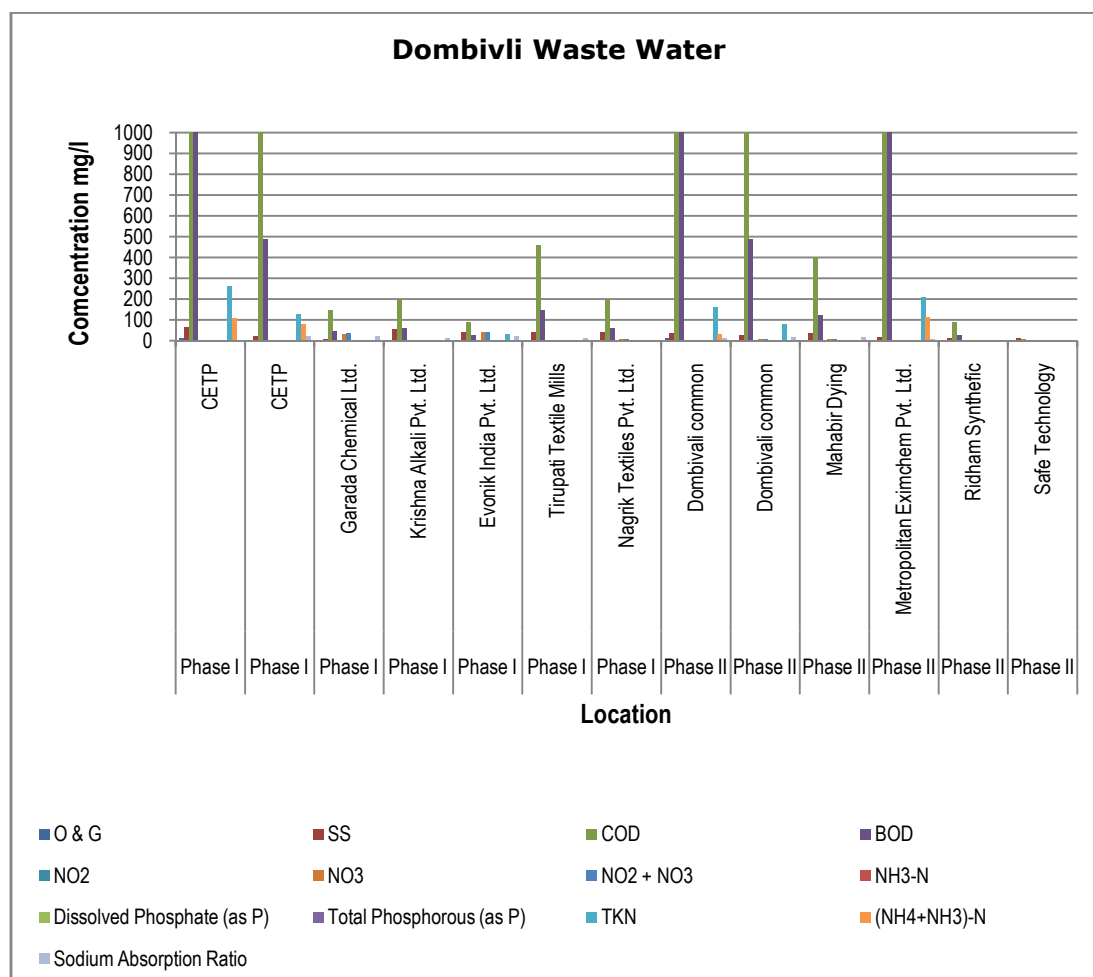
Graphs: Water/Waste Water Quality Monitoring for Dombivli MIDC:
