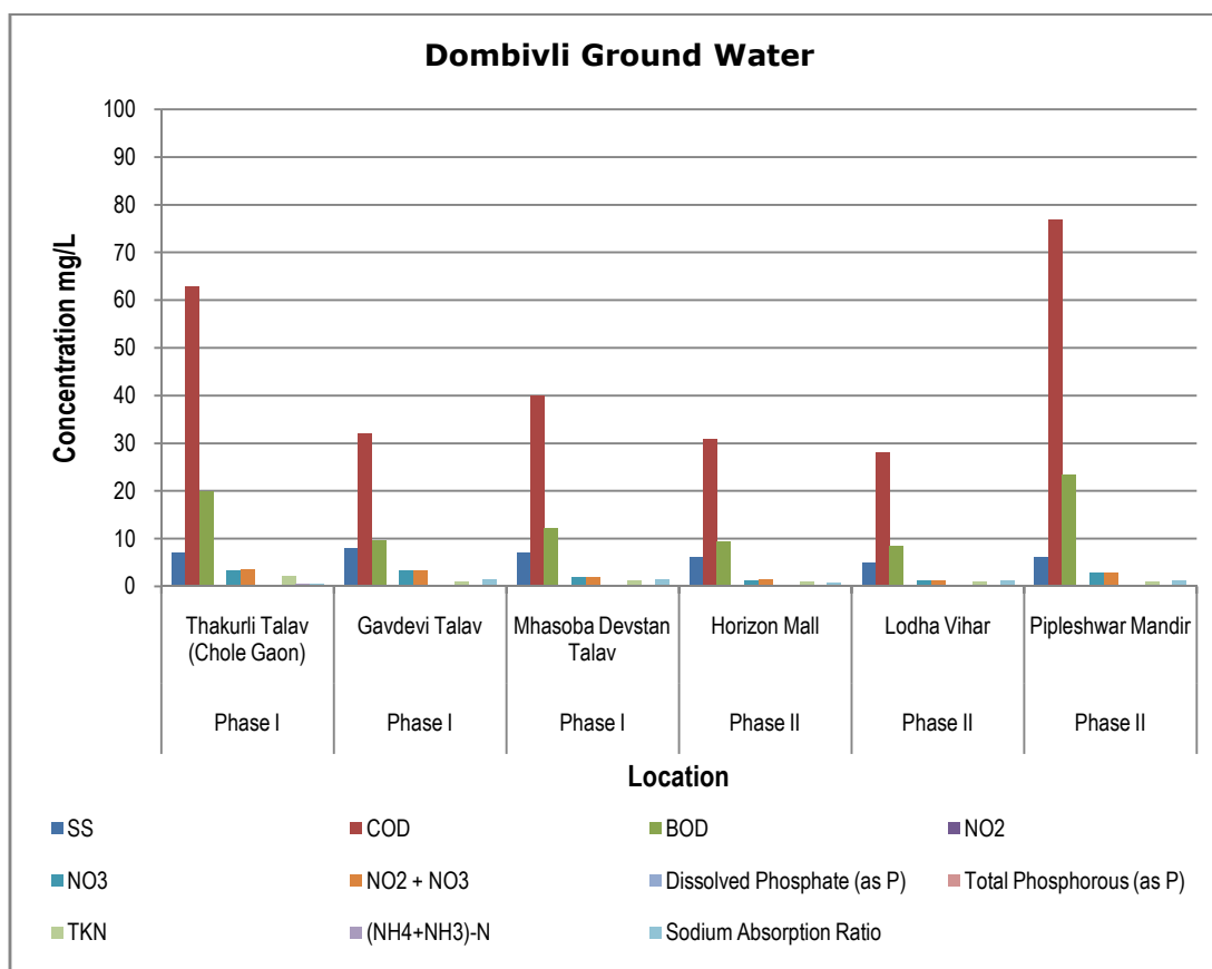
Graphs: Ground Water Quality Monitoring for Dombivli MIDC:
