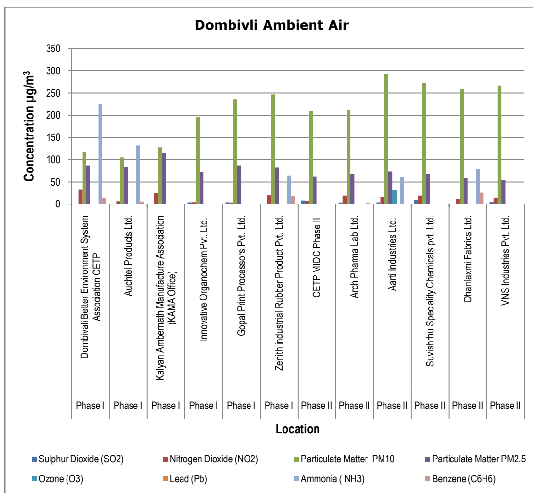
Graphs: Ambient Air Quality Monitoring for Dombivli MIDC:
