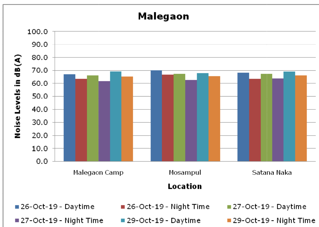
Chart 4.23: Noise Levels during Diwali Festival, 2019 in Malegaon
