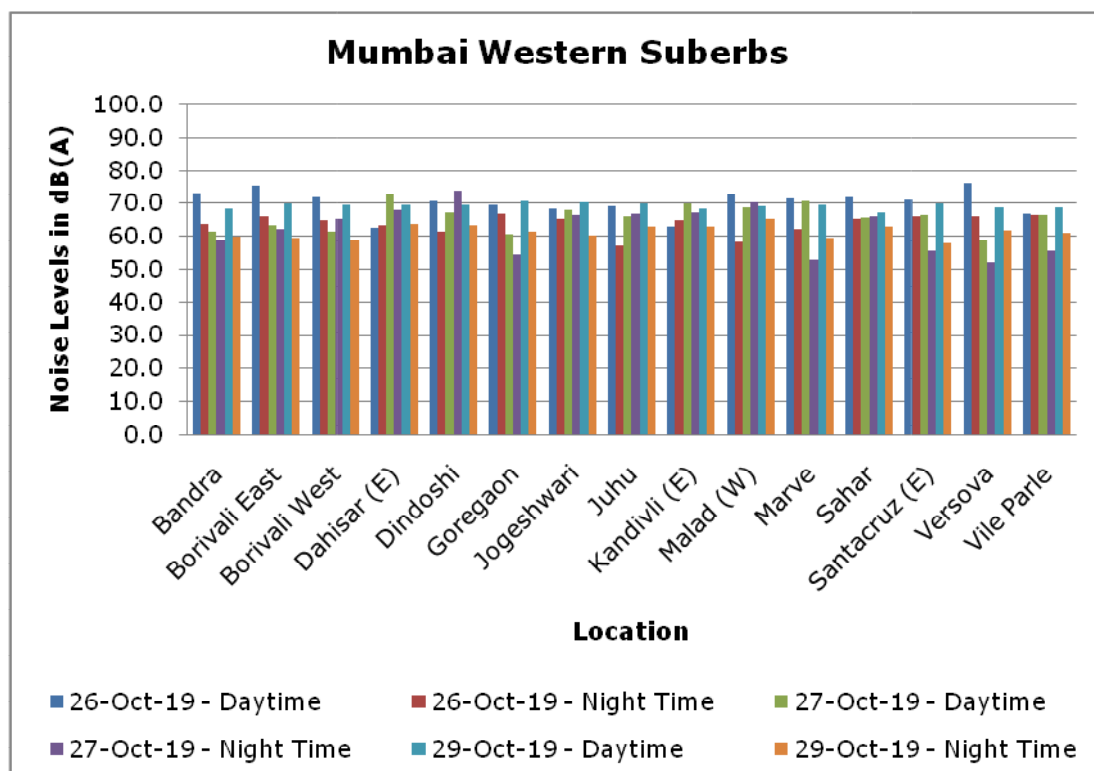
Chart 4.2: Noise Levels during Diwali Festival, 2019 in Mumbai Western Suberbs
