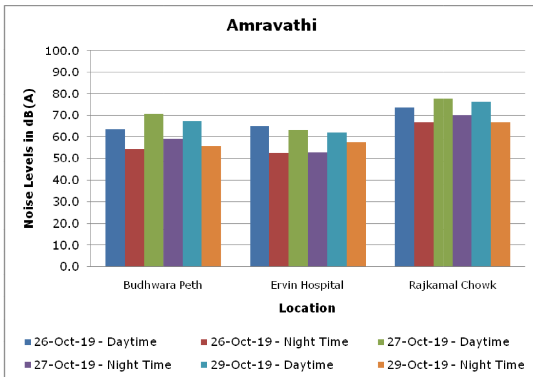
Chart 4.11: Noise Levels during Diwali Festival, 2019 in Amravati
