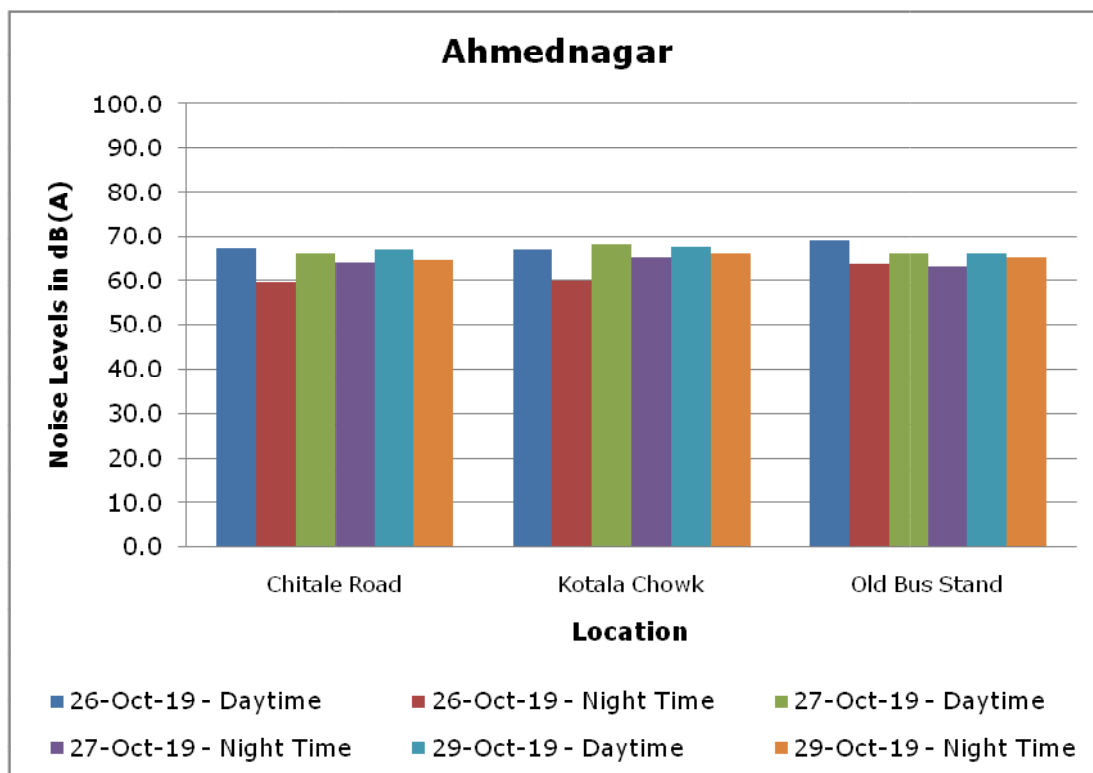
Chart 4.21: Noise Levels during Diwali Festival, 2019 in Ahmednagar
