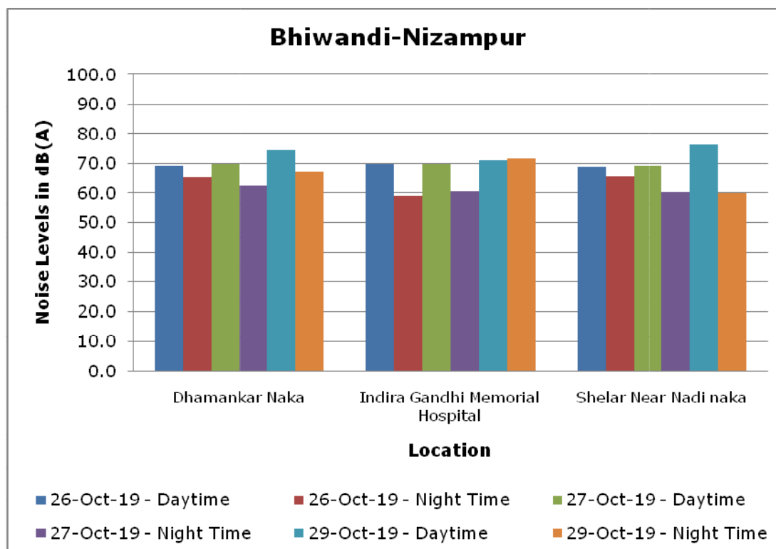
Chart 4.18: Noise Levels during Diwali Festival, 2019 in Bhiwandi-Nizampur
