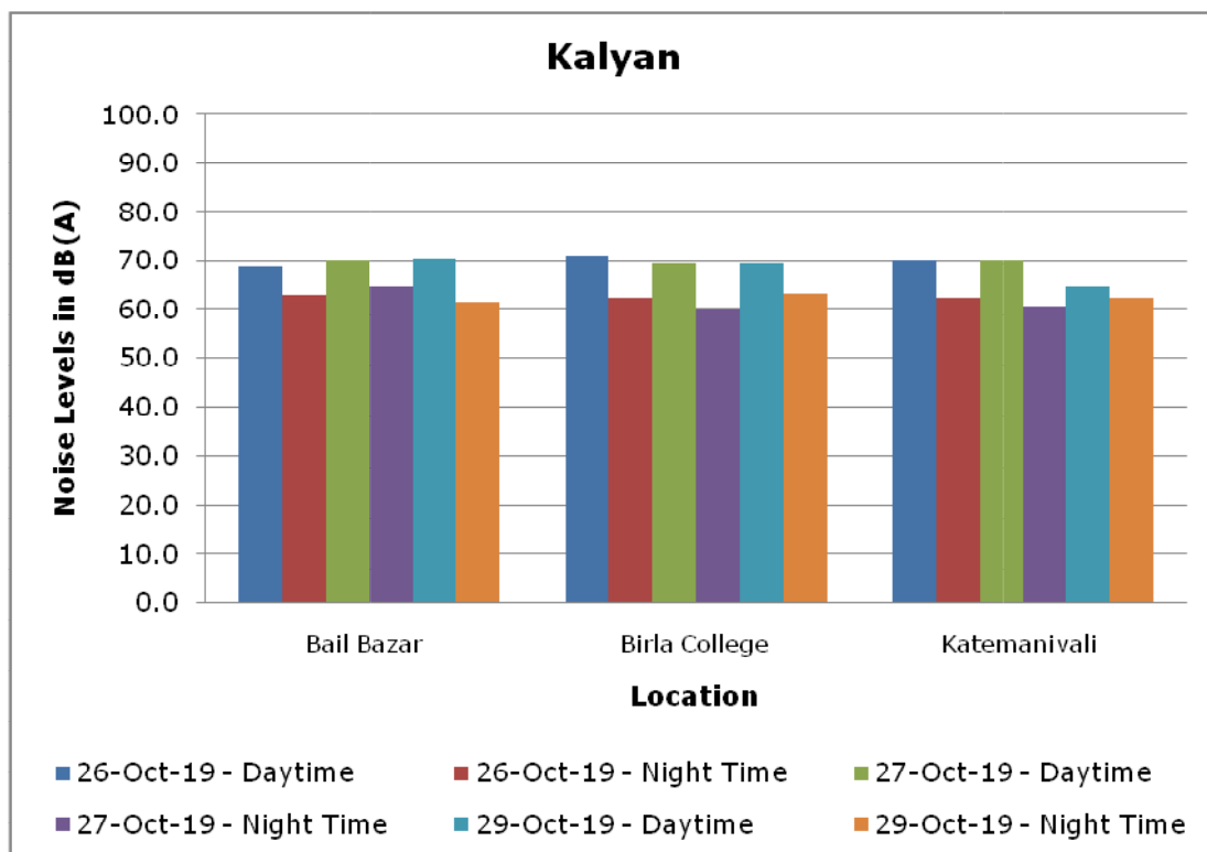
Chart 4.10: Noise Levels during Diwali Festival, 2019 in Kalyan
