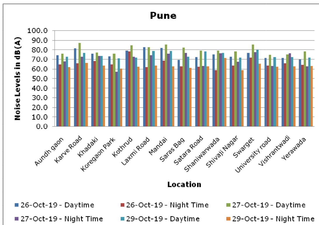
Chart 4.6: Noise Levels during Diwali Festival, 2019 in Pune
