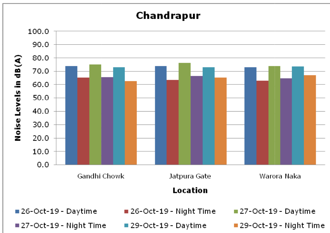
Chart 4.19: Noise Levels during Diwali Festival, 2019 in Chandrapur
