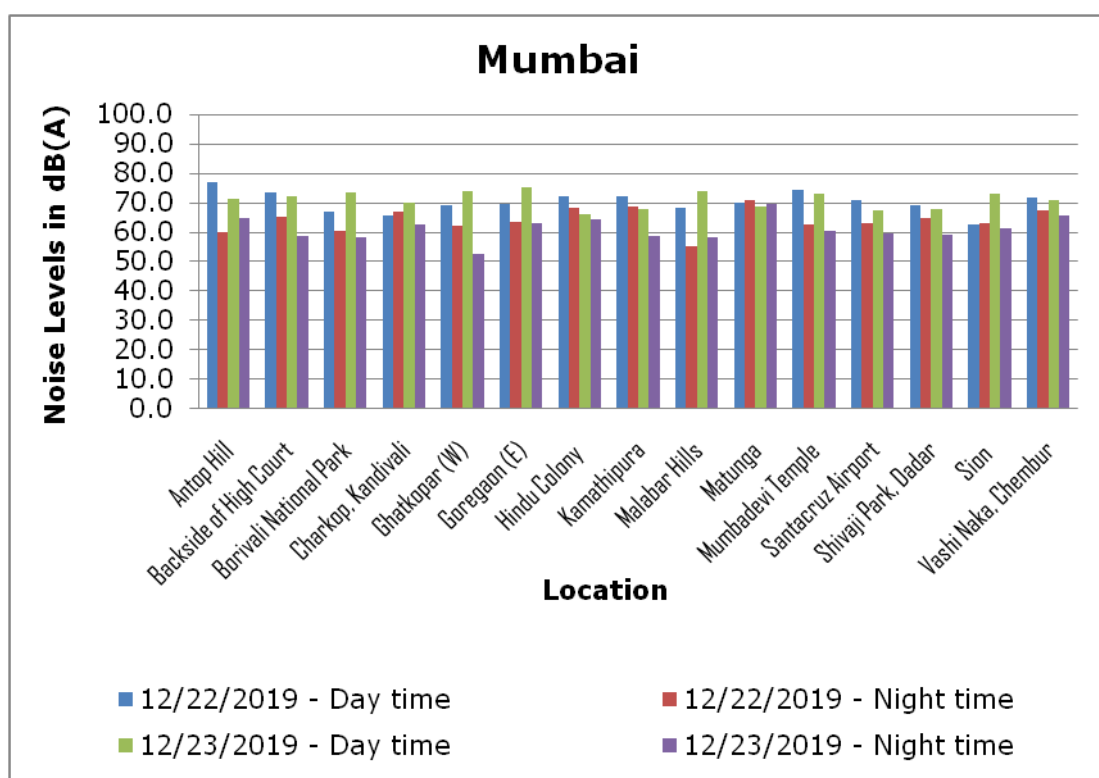
Chart 4.1: Noise Levels in Mumbai
