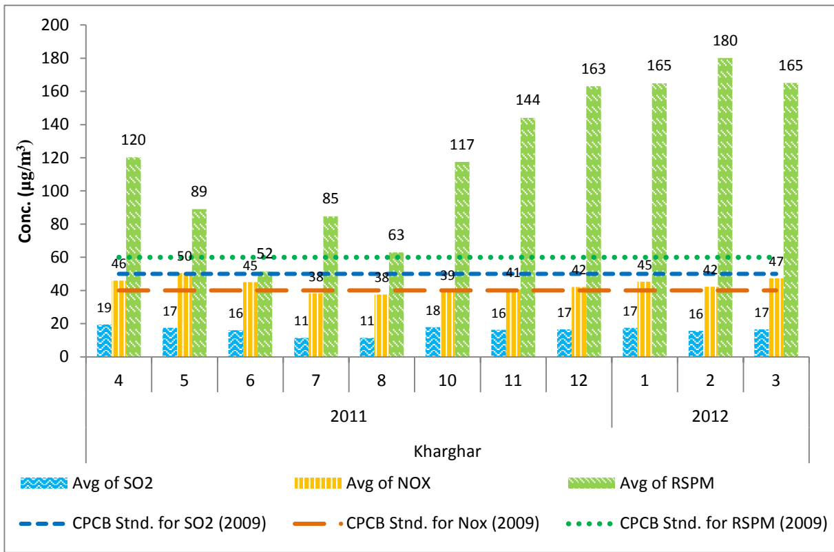
Figure No 131: Monthly average reading recorded at Kharghar - CIDCO Nodal Office - Talaja
