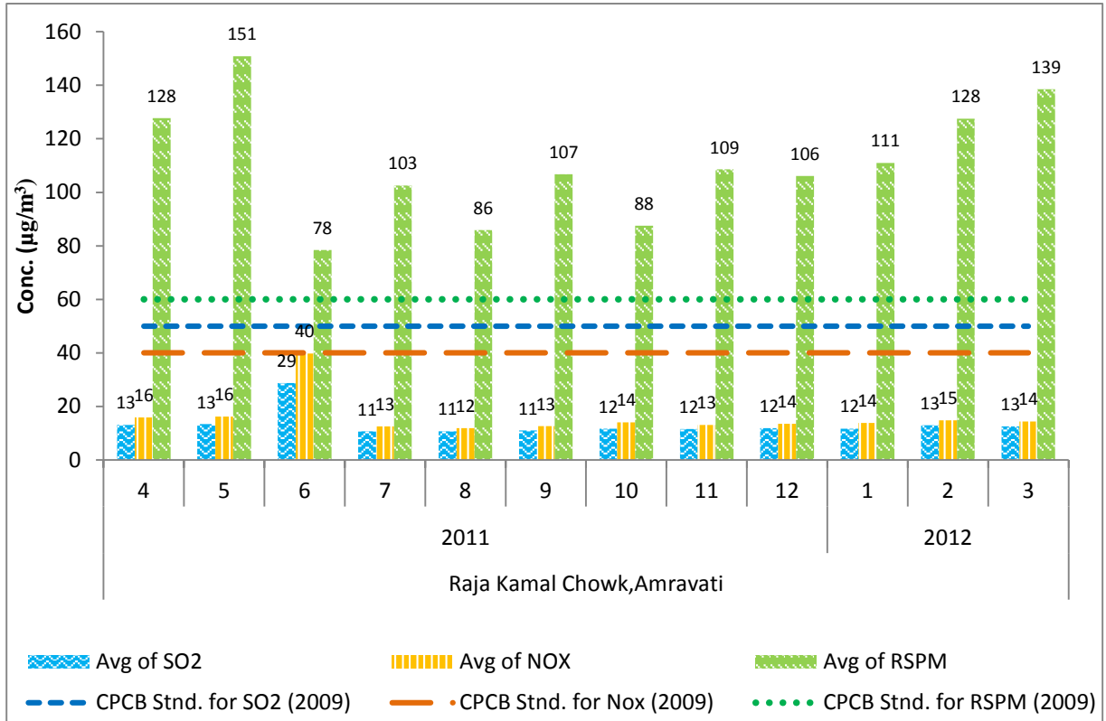
Figure No 31: Monthly average reading recorded at Raja Kamal Chowk, Amravati
