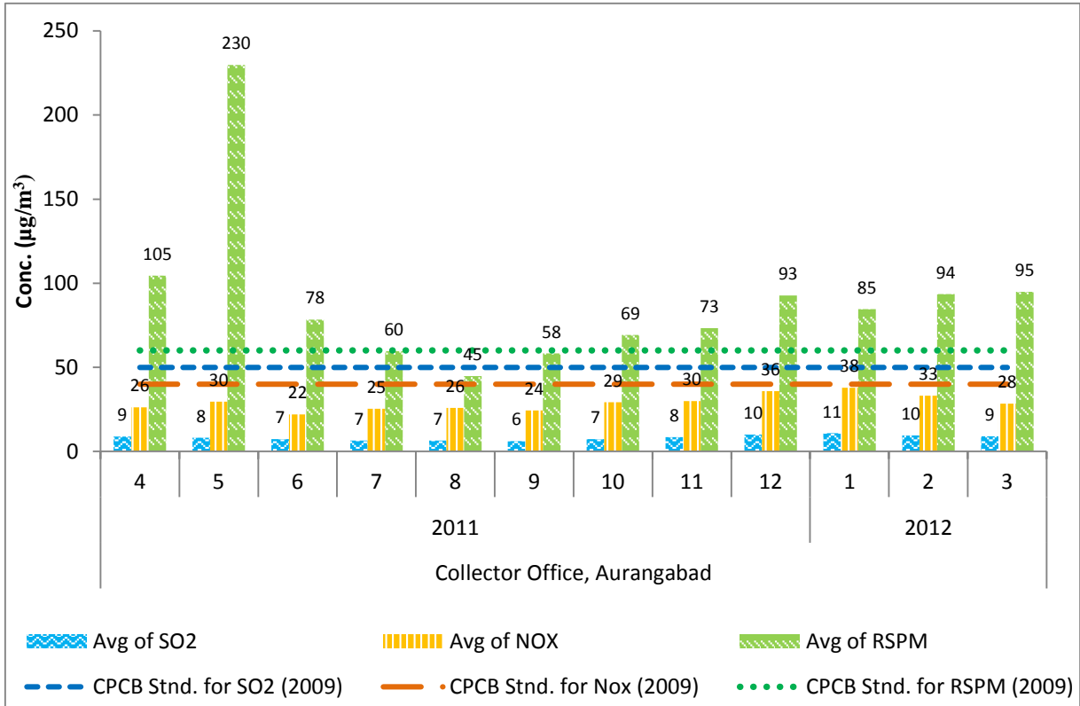
Figure No 35: Monthly average reading recorded at Collector Office, Aurangabad
