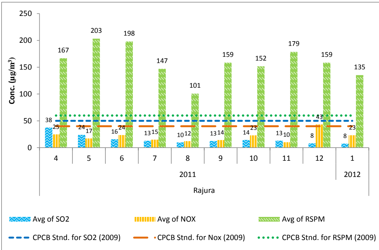
Figure No 61: Monthly average reading recorded at Rajura, Chandrapur
