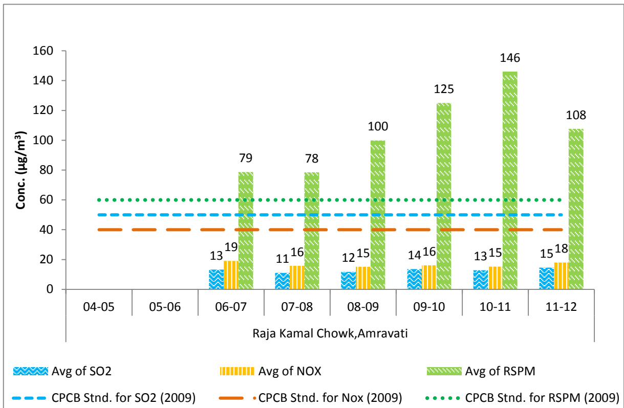
Figure No 32: Annual average trend of SO 2 , NO x and RSPM at Raja Kamal Chowk, Amravati
