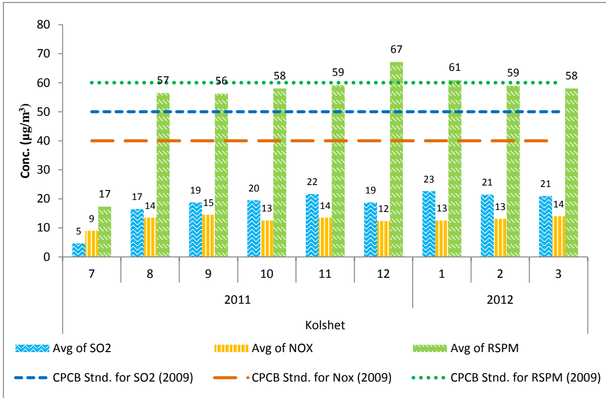
Figure No 153: Monthly average reading recorded at Kolshet - Thane
