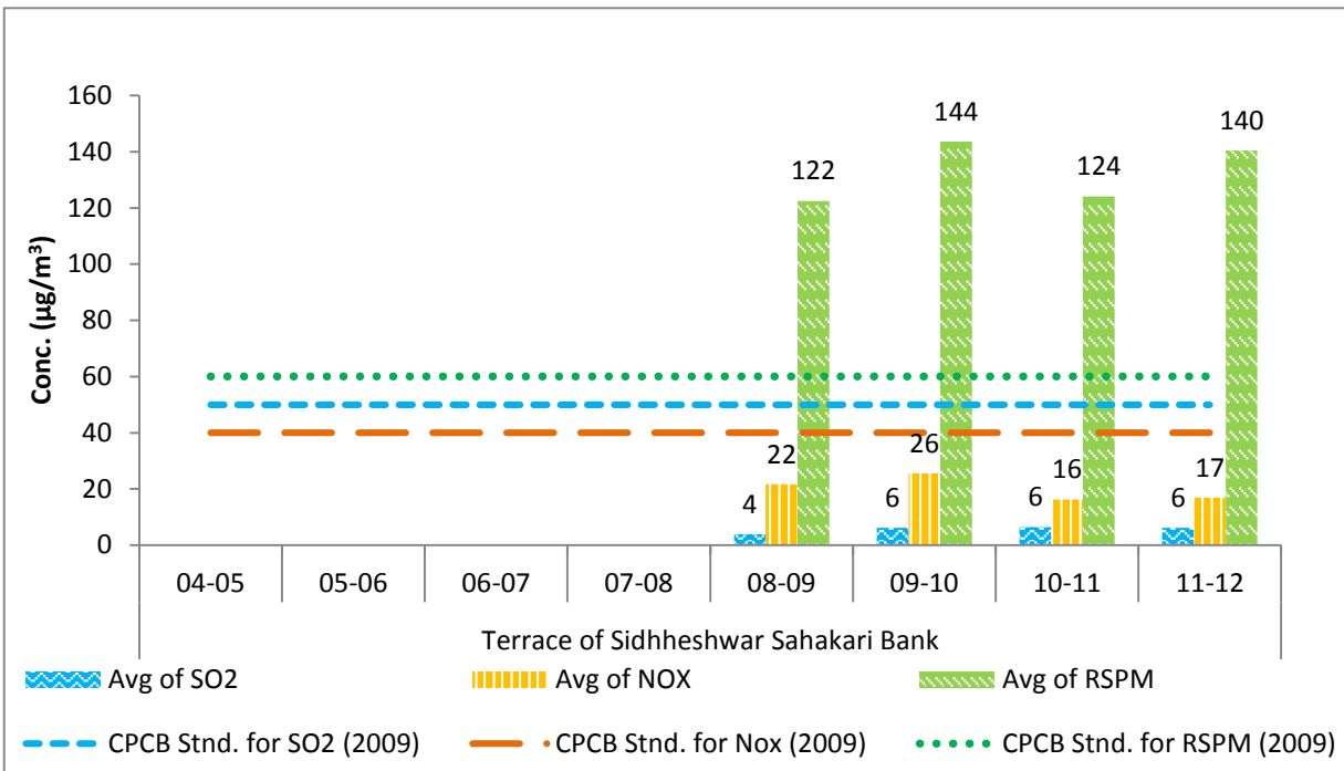
Figure No 48: Annual average trend of SO 2 , NO x and RSPM at Ganj Golai - Sidhshwar Bank - Latur
