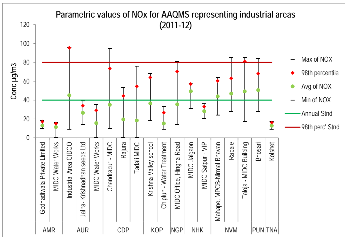
Figure No 10: Parametric values of NO x for AAQMS representing industrial areas (2011-12)
