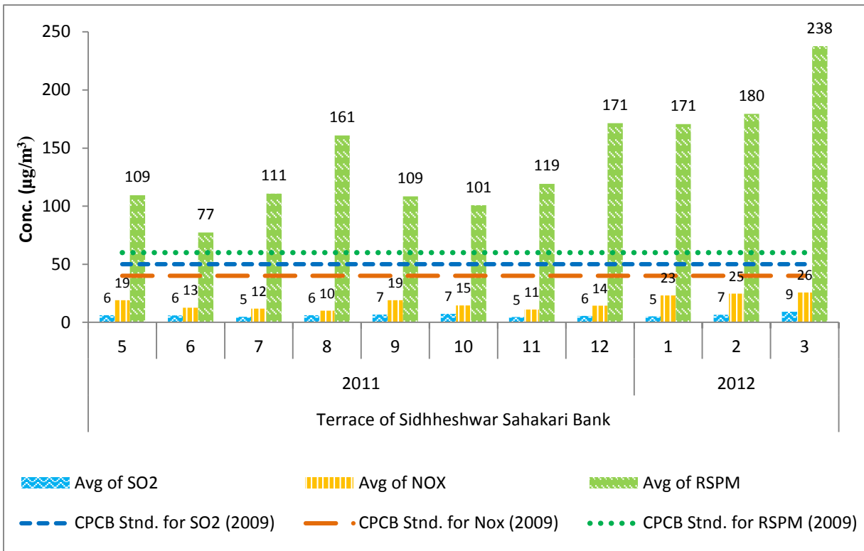
Figure No 47: Monthly average reading recorded at Ganj Golai - Sidhshwar Bank - Latur
