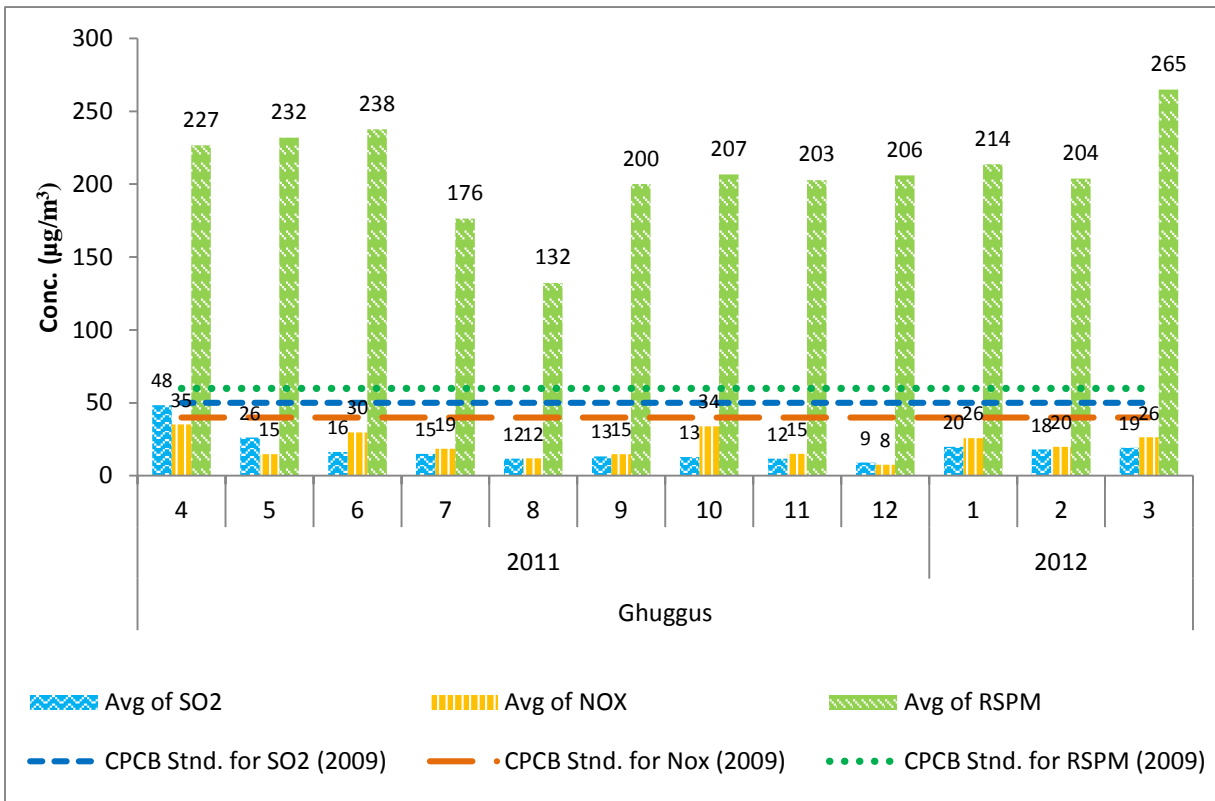
Figure No 53: Monthly average reading recorded at Ghuggus – Chandrapur
