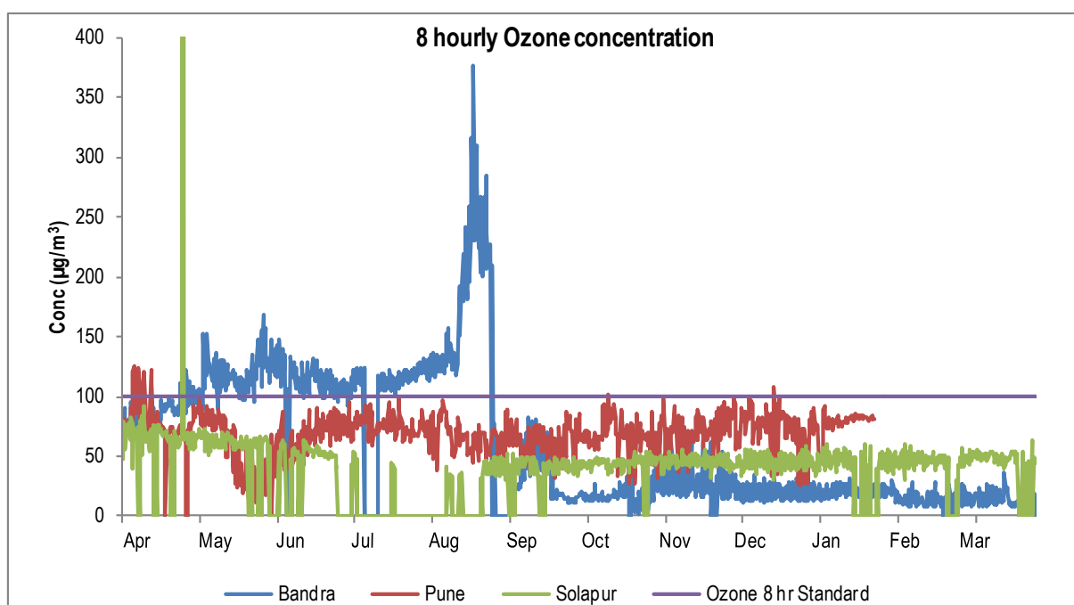
Figure No. 24: Ozone concentrations at Bandra, Pune and Solapur (2013-14)
