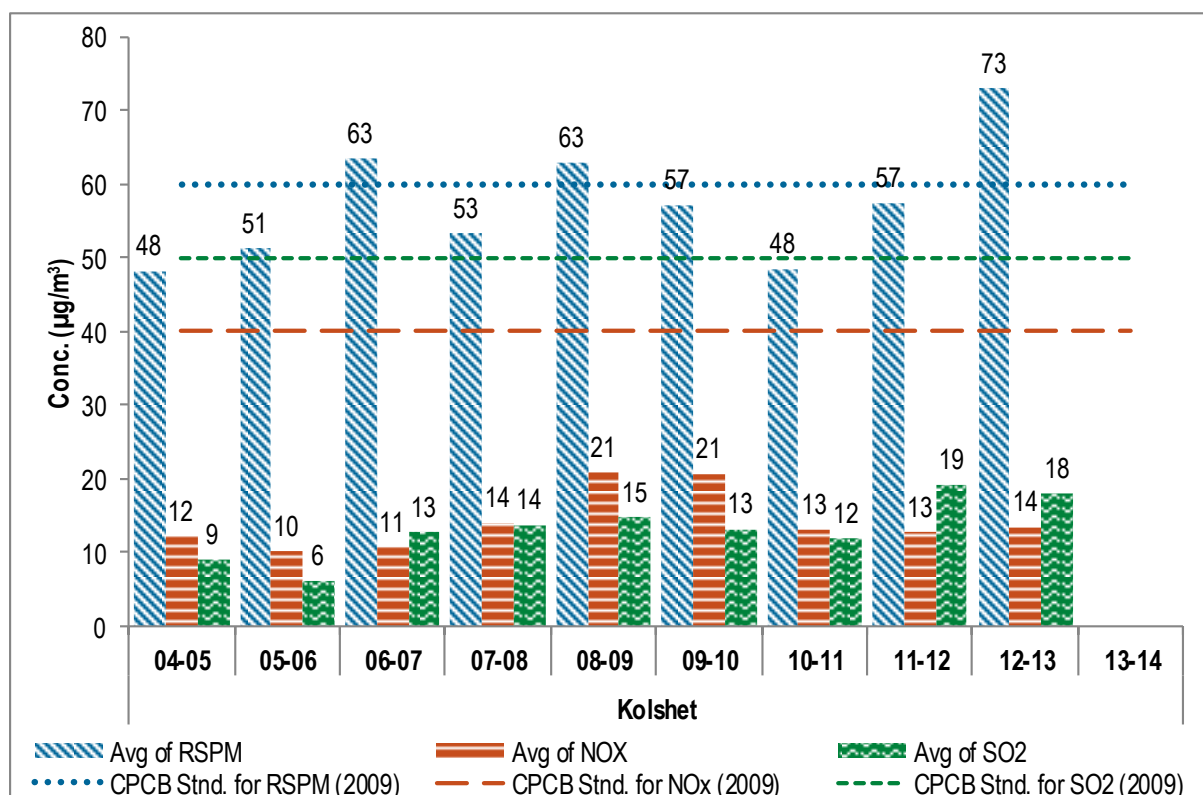
Figure No. 187: Annual average trend of SO 2 , NO x and RSPM at Kolshet
