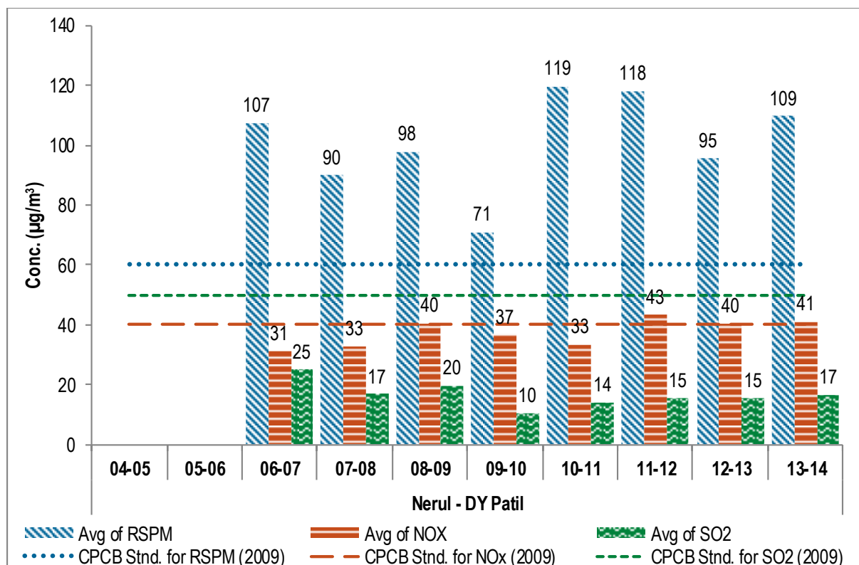
Figure No. 150: Annual average trend of SO 2 , NO x and RSPM at Nerul - DY Patil
