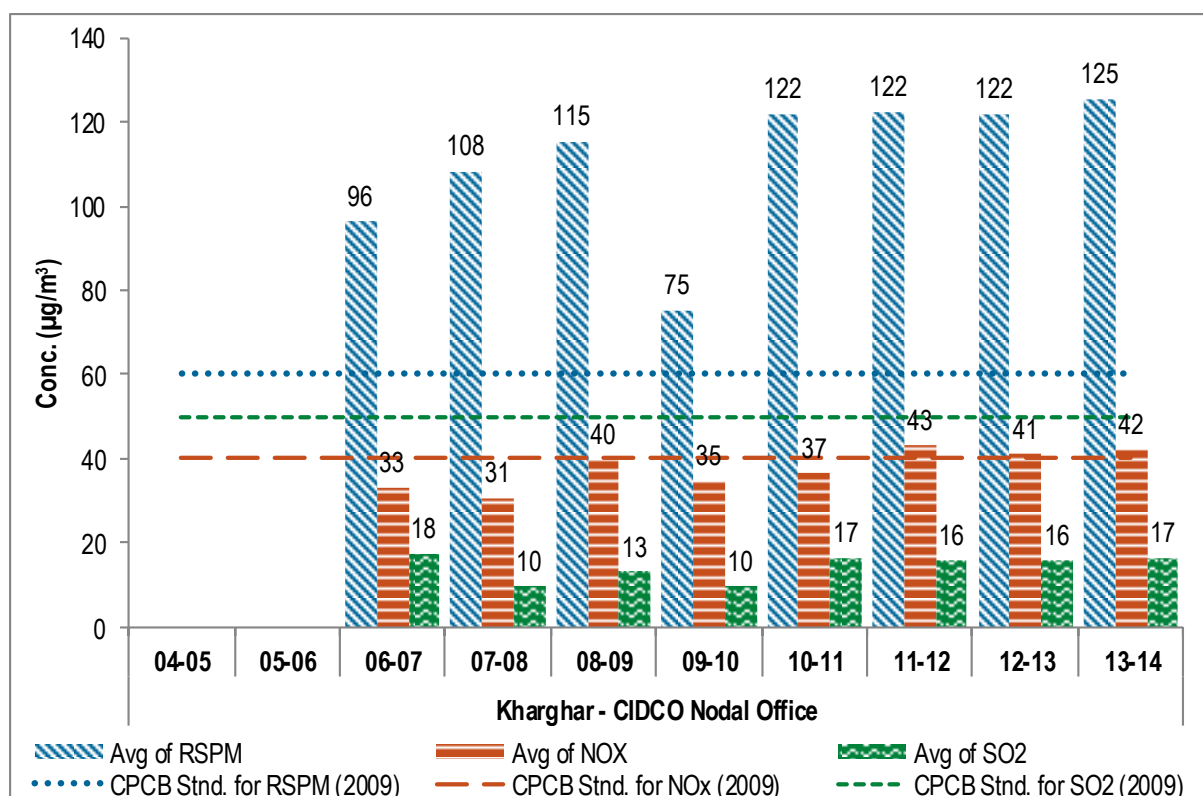
Figure No. 158: Annual average trend of SO 2 , NO x and RSPM at Kharghar - CIDCO Nodal Office
