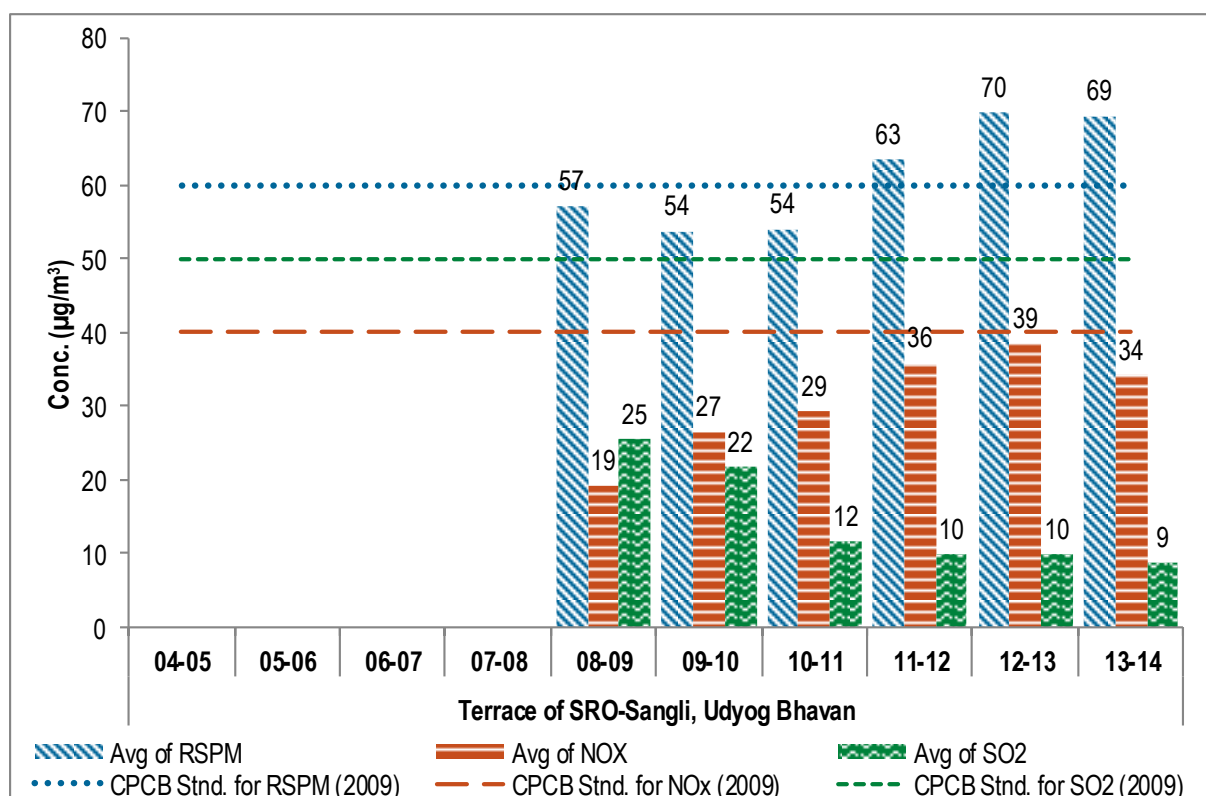
Figure No. 110: Annual average trend of SO 2 , NO x and RSPM at -Terrece of SRO-Sangli, Udyog Bhavan
