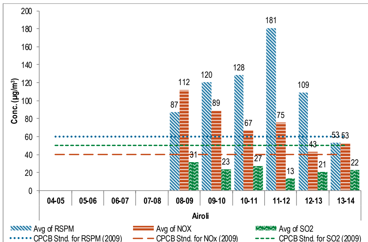
Figure No. 154: Annual average trend of SO 2 , NO x and RSPM at -Airoli
