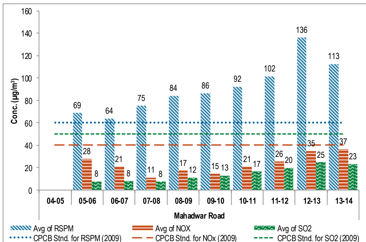
Figure No. 108: Annual average trend of SO 2 , NO x and RSPM at -Mahadwar Road
