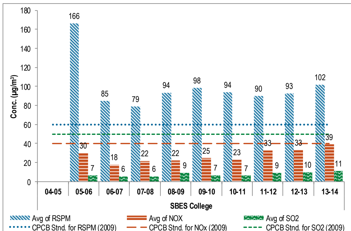
Figure No. 45: Annual average trend of SO 2 , NO x and RSPM at SBES College – Aurangabad
