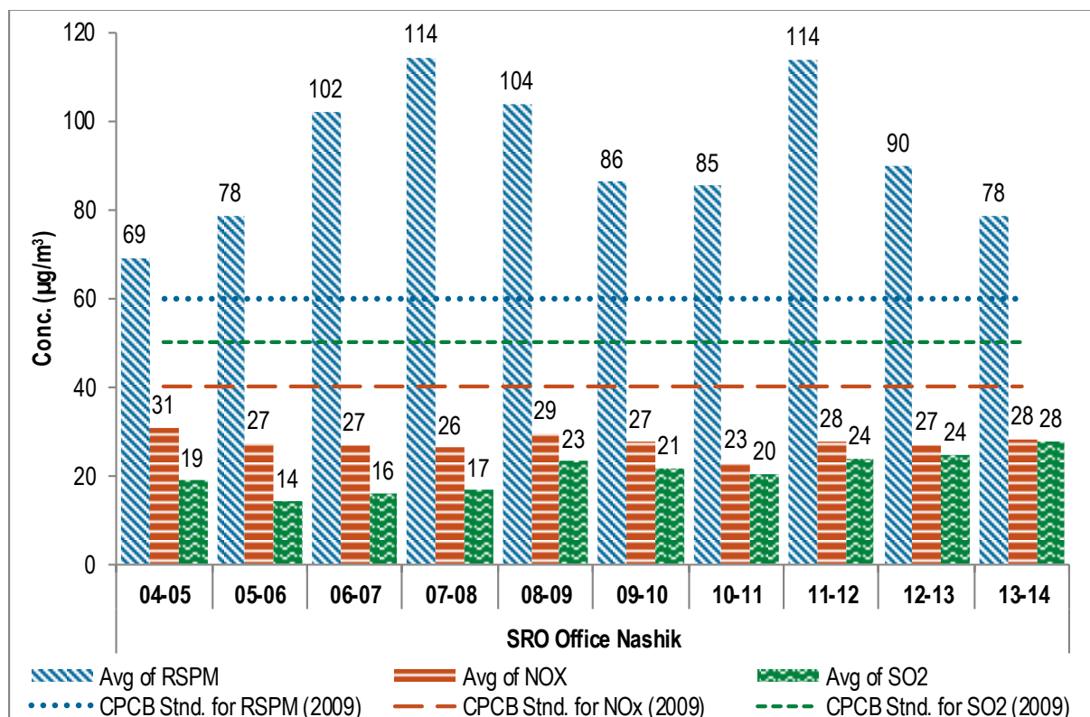
Figure No. 145: Annual average trend of SO 2 , NO x and RSPM at -SRO Office Nashik
