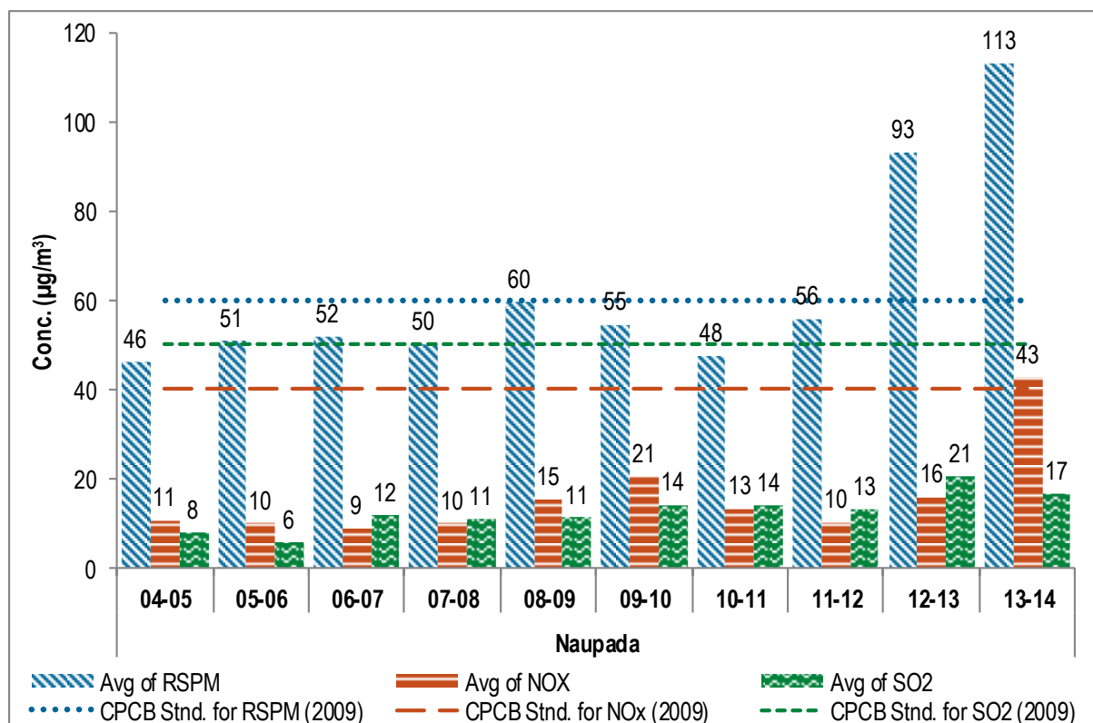
Figure No. 185: Annual average trend of SO 2 , NO x and RSPM at Naupada
