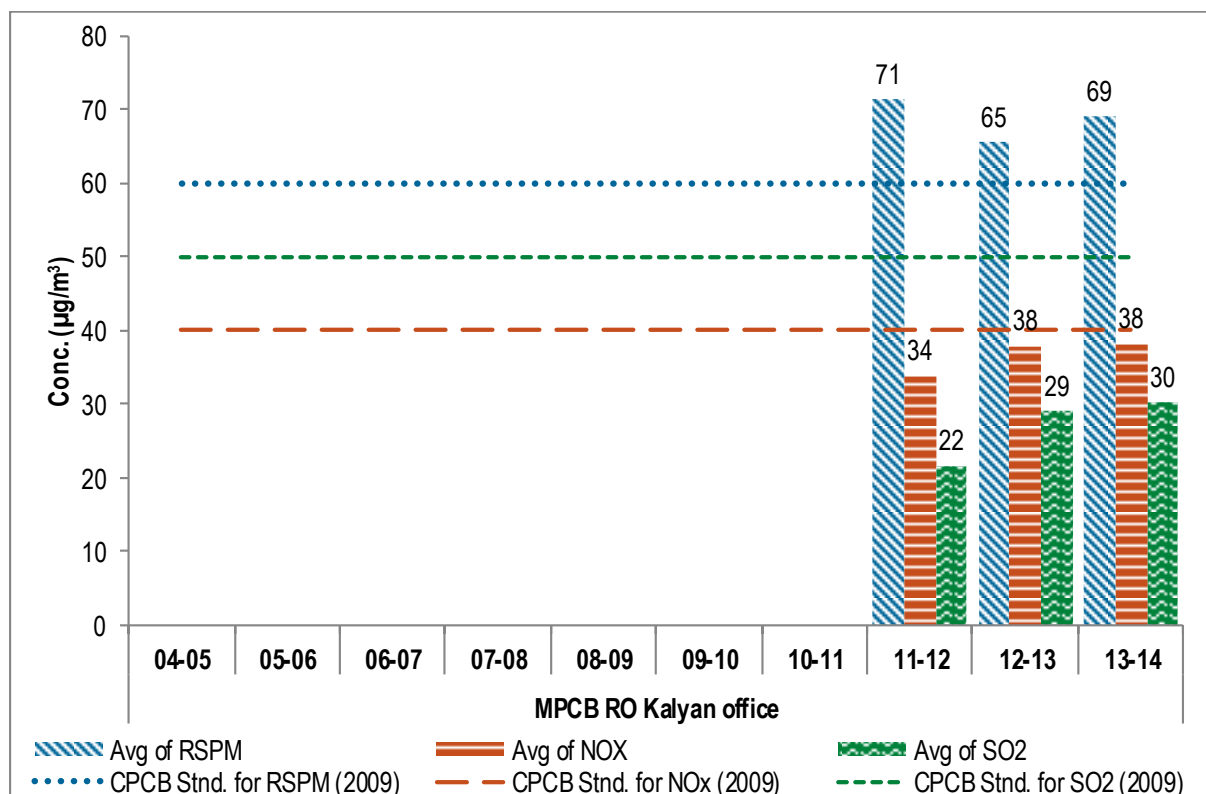
Figure No. 93: Annual average trend of SO 2 , NO x and RSPM at MPCB RO Kalyan Office
