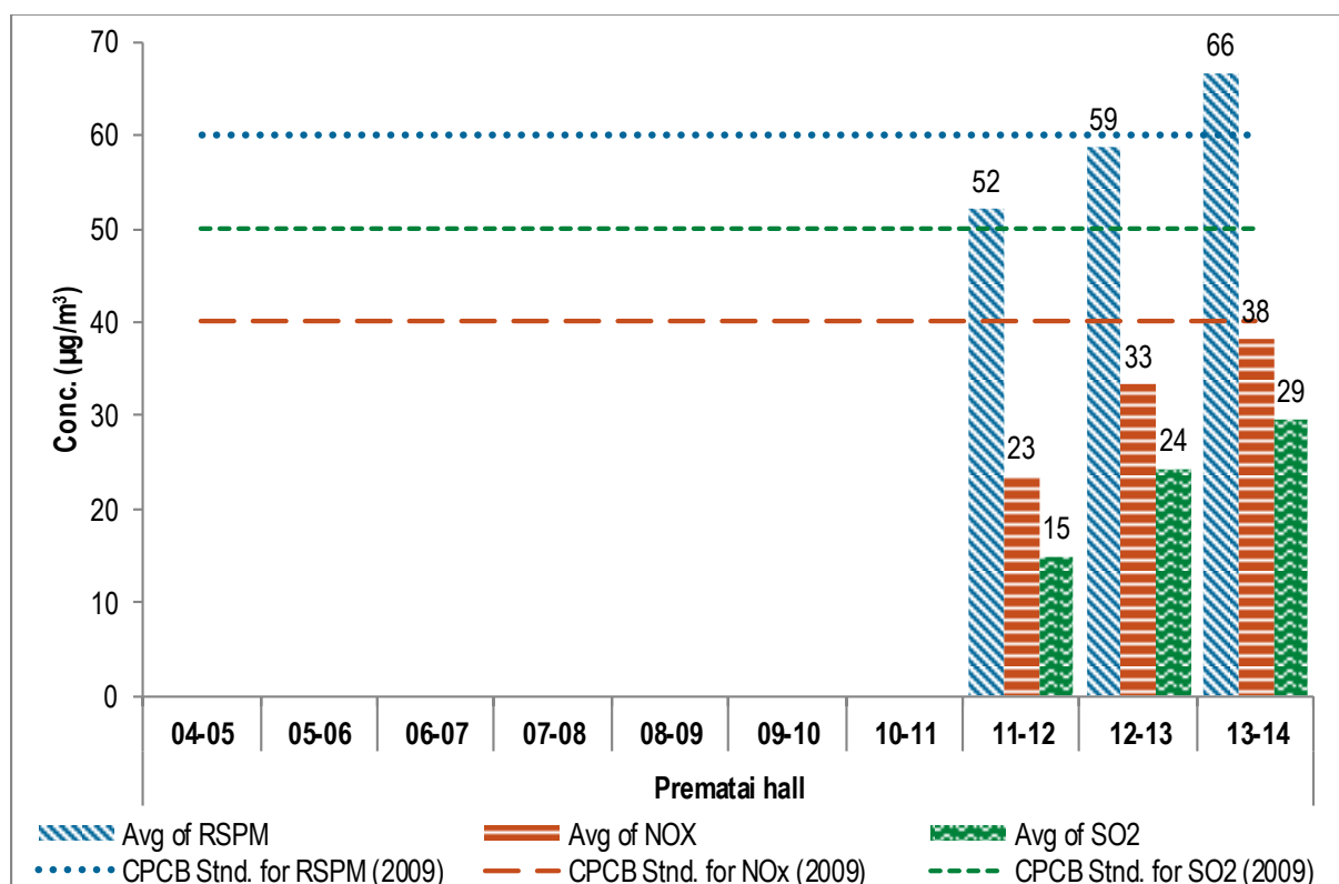
Figure No. 87: Annual average trend of SO 2 , NO x and RSPM at Premataihall -Bhiwandi
