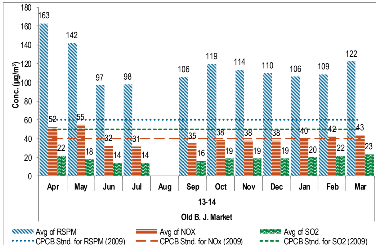
Figure No. 132: Monthly average reading recorded at- Old B. J. Market
