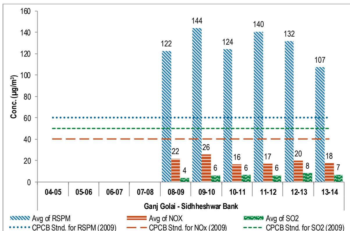
Figure No. 59: Annual average trend of SO 2 , NO x and RSPM at Ganj Golai Sidhsheshwar Bank
