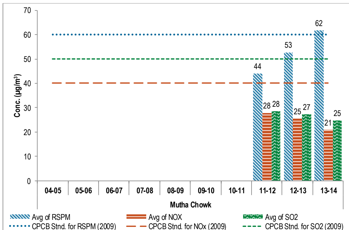
Figure No. 63: Annual average trend of SO 2 , NO x and RSPM at Mutha Chowk
