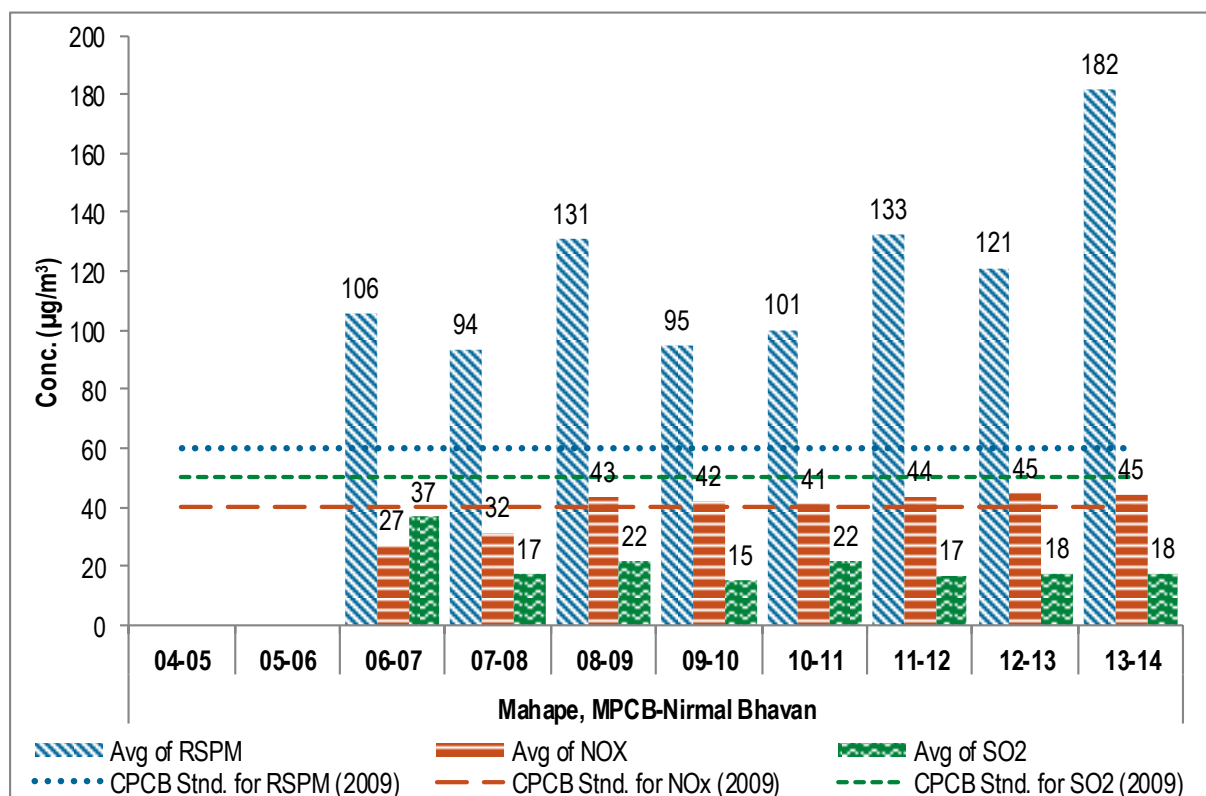
Figure No. 152: Annual average trend of SO 2 , NO x and RSPM at Mahape, MPCB-Nirmal Bhavan
