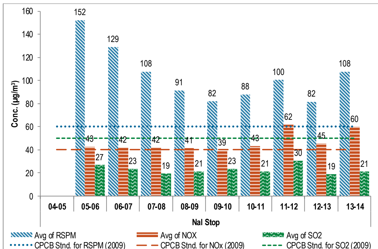
Figure No. 165: Annual average trend of SO 2 , NO x and RSPM at Nal Stop
