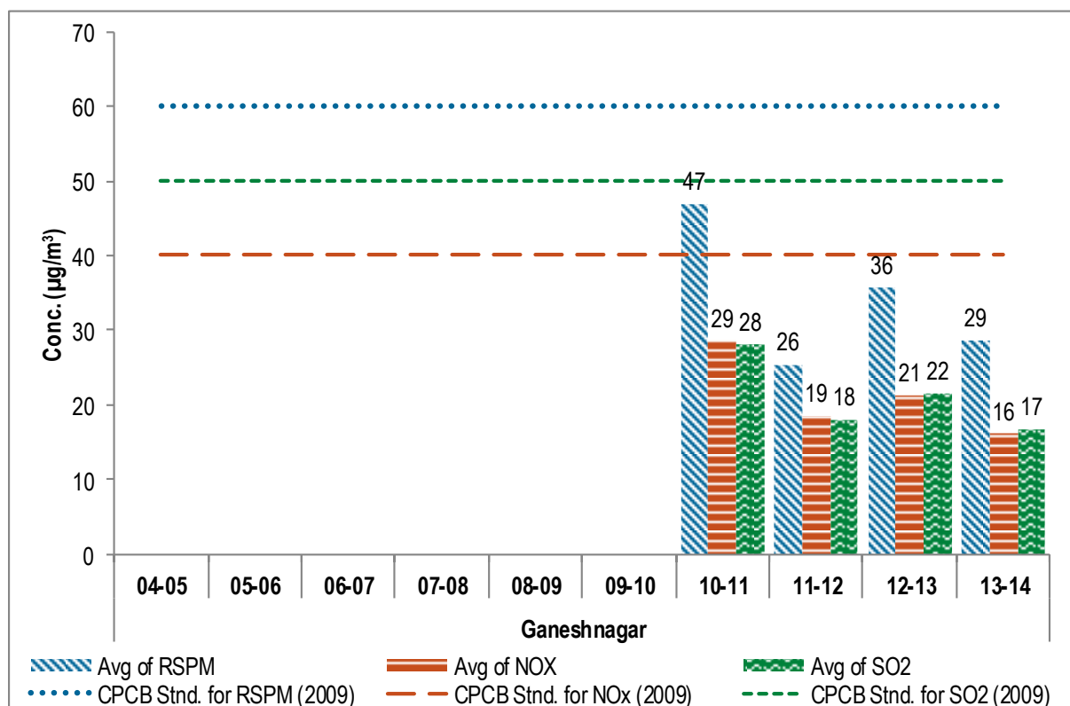
Figure No. 61: Annual average trend of SO 2 , NO x and RSPM at Ganeshnagar
